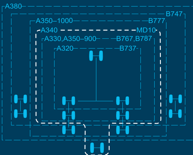
COMMON COMMERCIAL AIRCRAFT TRICYCLE AND EXTENDED TRICYCLE
